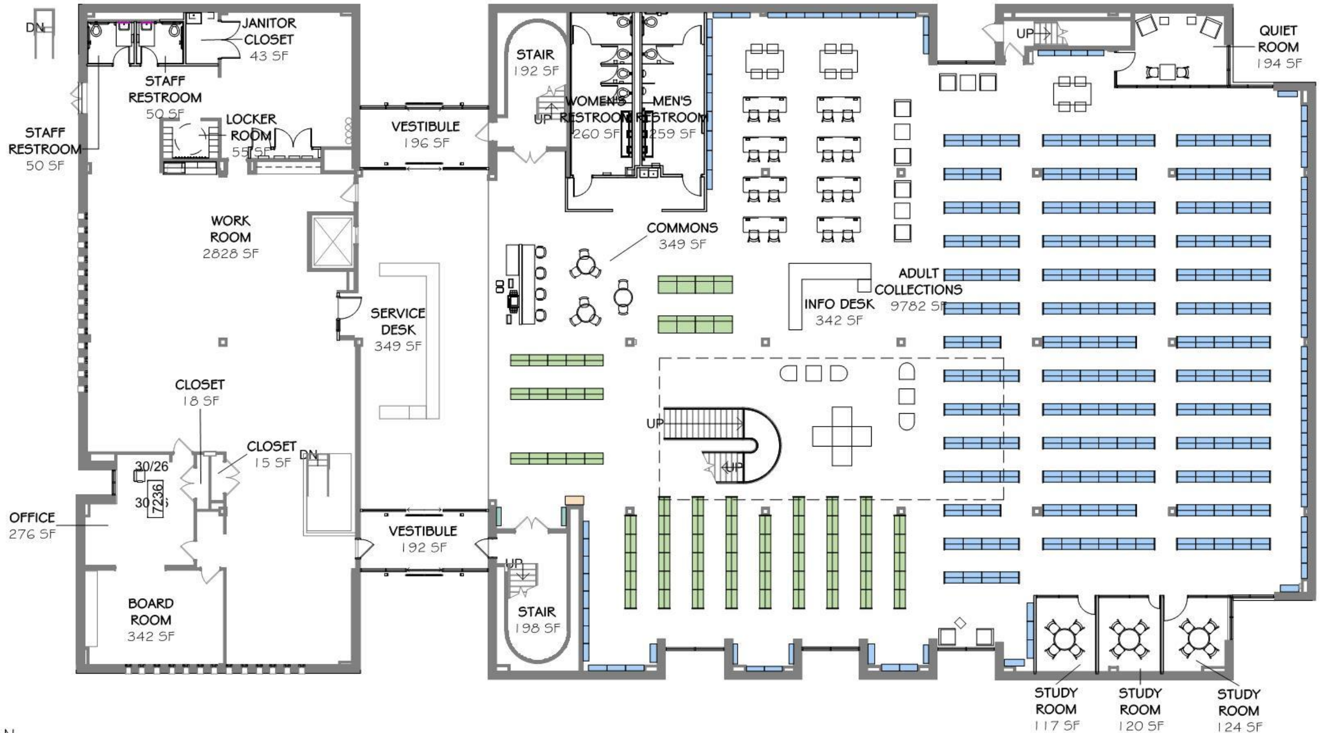
FIRST FLOOR PLAN 1/16" = 1'-0"
